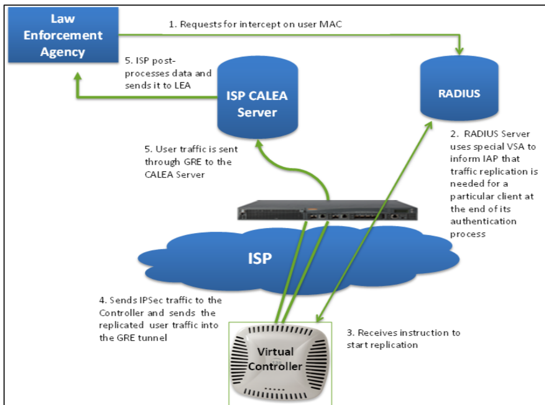
Figure 106 IAP to CALEA Server through VPN
